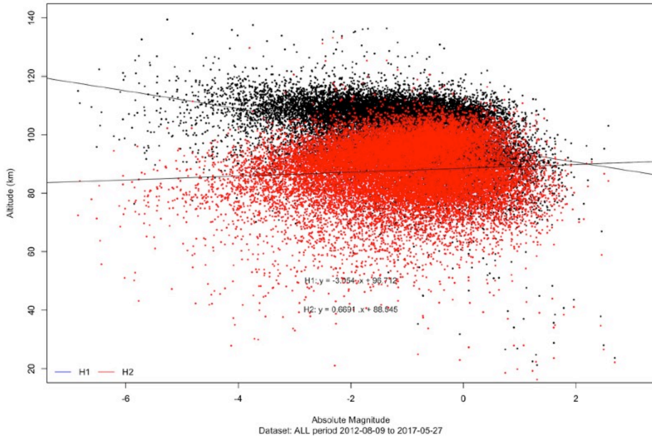
Absolute magnitude vs H1 / H2 (All streams and sporadics)
