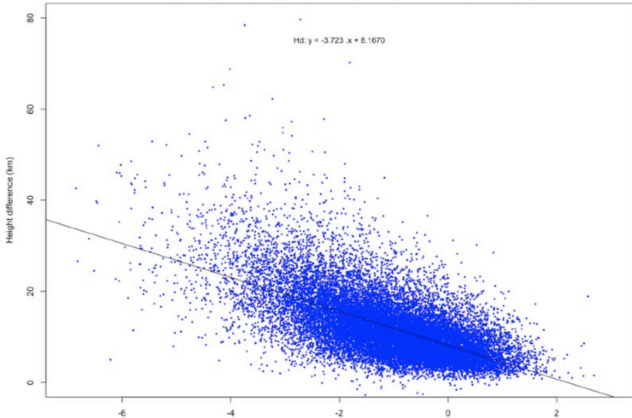
Absolute magnitude vs height difference (H1 - H2) (All streams and sporadics)
