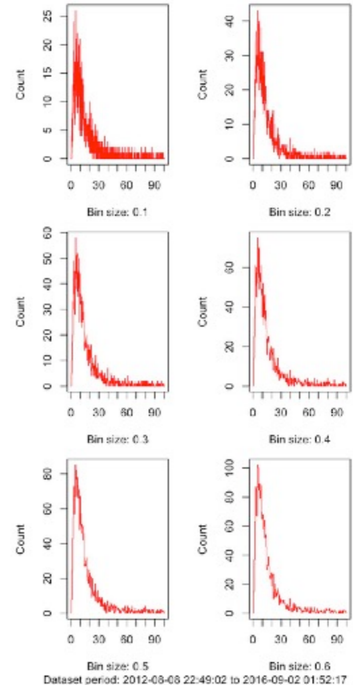
Frequency distribution of (a) (Perseids)
