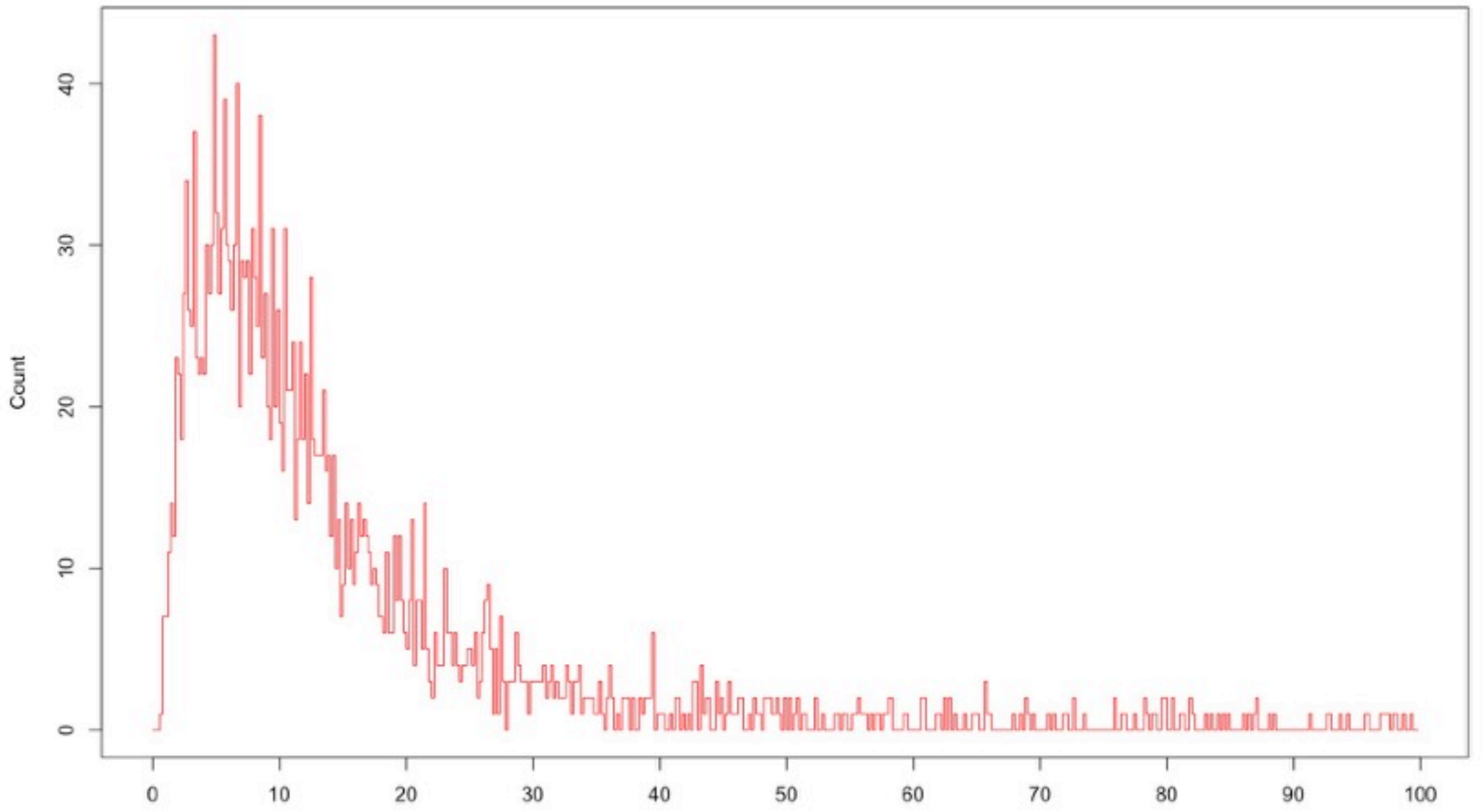
Semi-major Axis (au) Dataset: PER period 2012-08-09 to 2016-09-01
