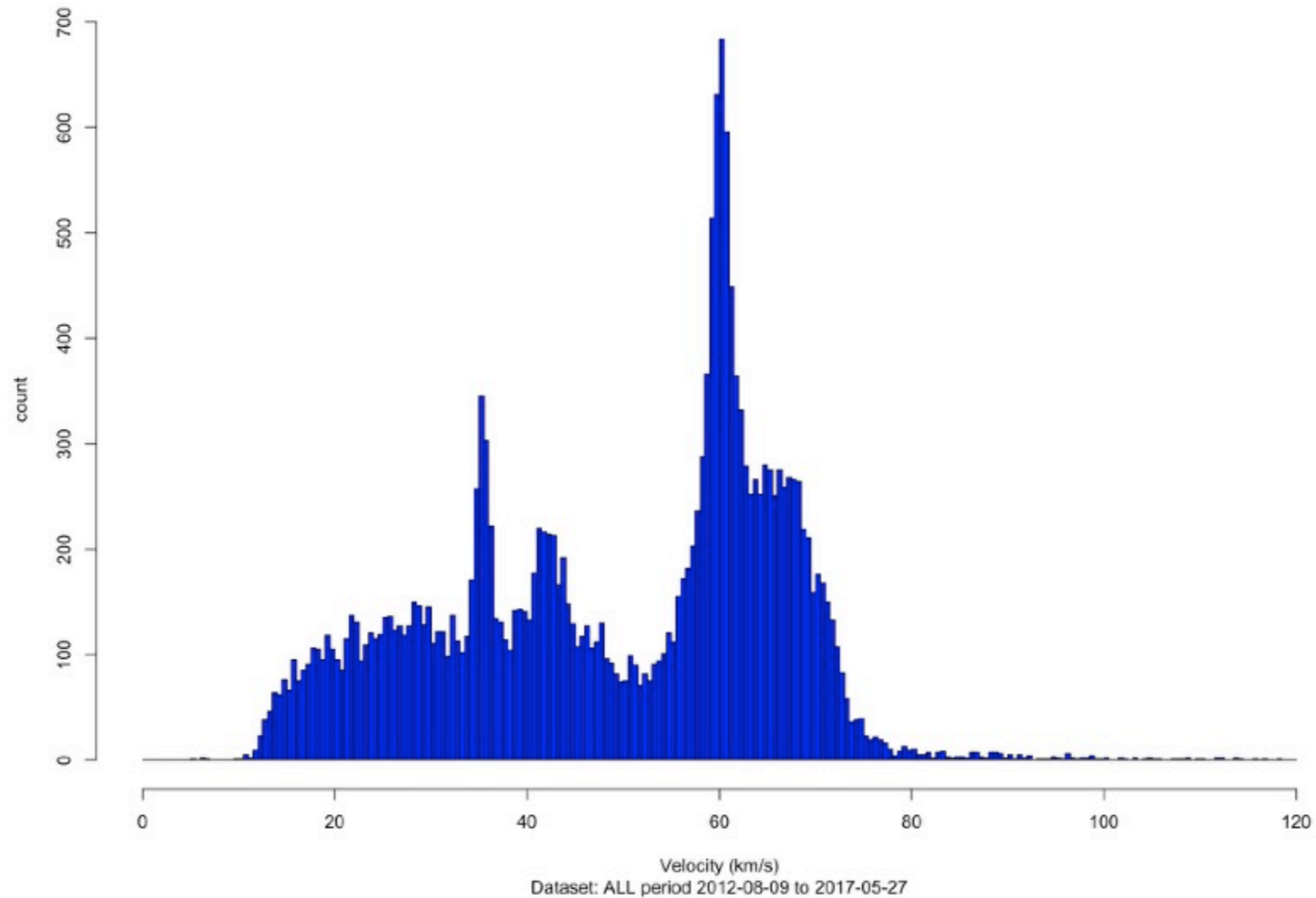
Velocity distribution (All streams and sporadics)
