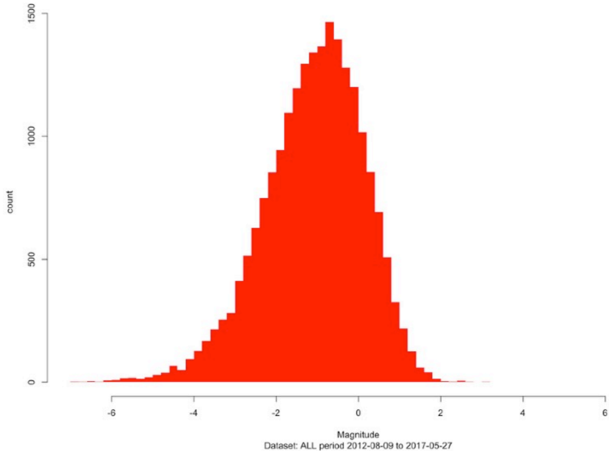
Magnitude distribution (All streams and sporadics)
