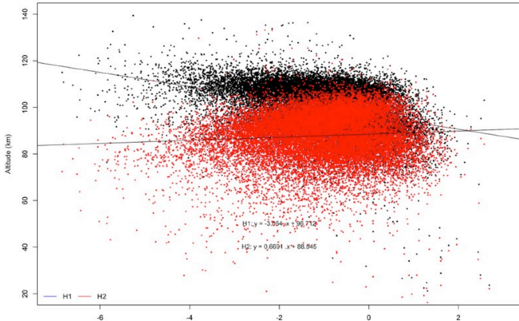
Absolute magnitude vs H1 / H2 (All streams and sporadics)
