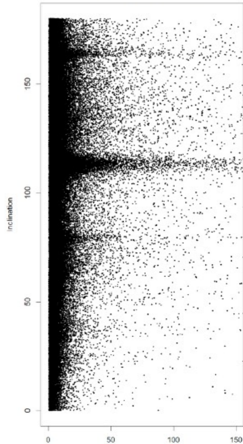
Semi-major axis vs Inclination (All streams and sporadics)
