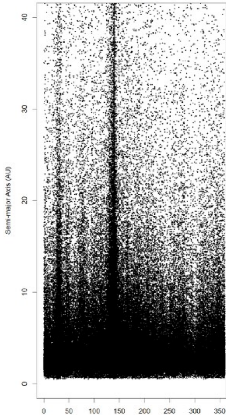
Longitude of Ascending Node vs Semi-major axis (All streams and sporadics)
